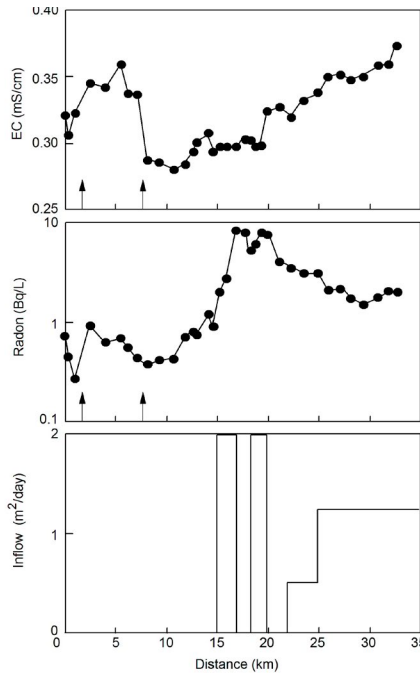
Figure 2. Groundwater inflow rates determined by the measurement of electrical conductivity and radon activity in the Cockburn River, New South Wales (Cook et al., 2006).
