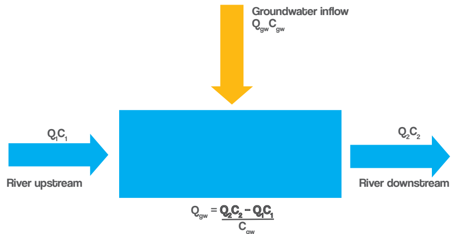
Figure 1. Conceptual model of how inflowing groundwater may be quantified from the change in concentration in river water ( Q_1 , Q_2 = flow upstream, downstream, C_1 , C_2 = concentration upstream, downstream, Q_{gw} , C_{gw} = groundwater inflow, groundwater concentration)
